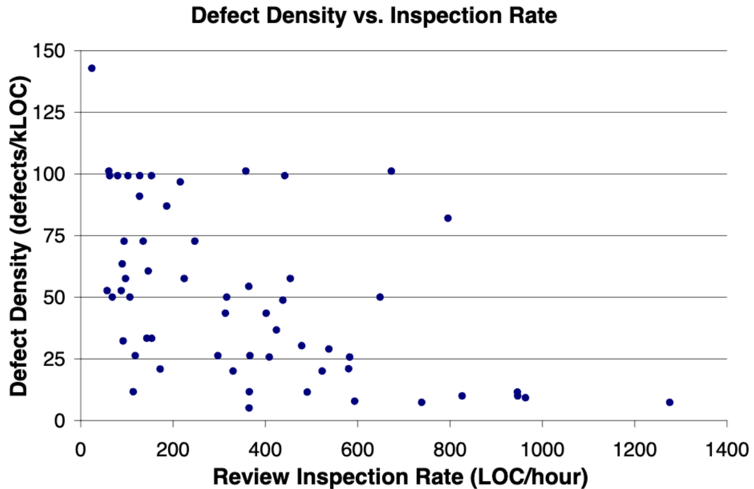
Figure 22: Reviewers become less effective at finding defects as their pace through the review accelerates.
